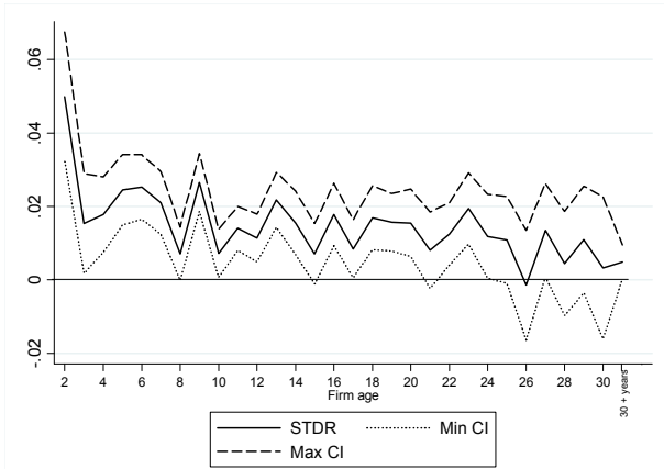
Figure 12: Sensitivity of firm growth to the short-term debt ratio – i.e. \gamma_2 from equation (3), for firms of different ages. LAD coefficient estimate, with 95% error bars.
